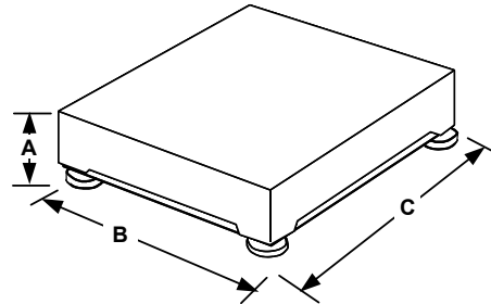
TrimWeigh III Base
